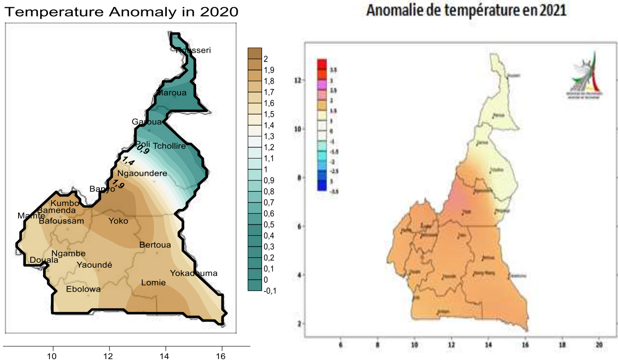
Figure 3- 6: Temperature anomaly in 2020 and 2021
