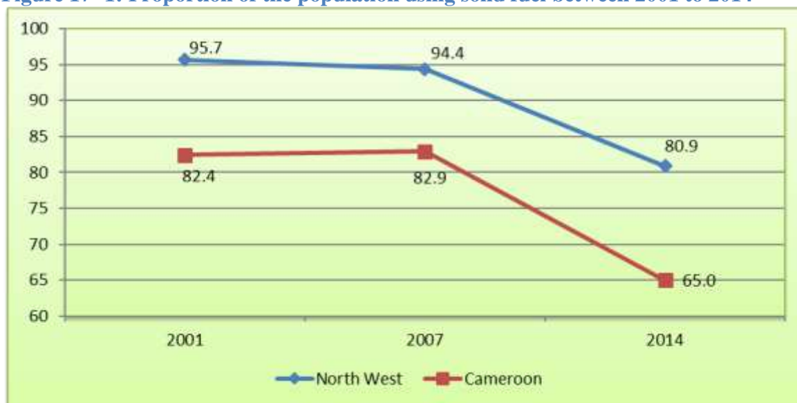
Figure 17- 1: Proportion of the population using solid fuel between 2001 to 2014
