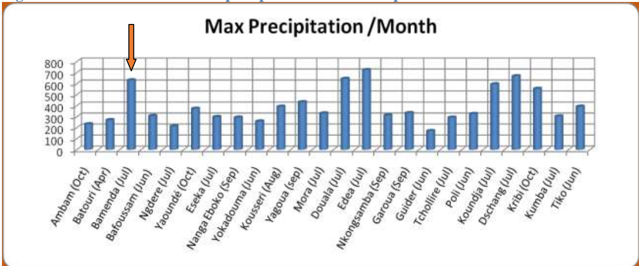
Figure 3- 2: Maximum observed precipitation at a station per month in 2020
